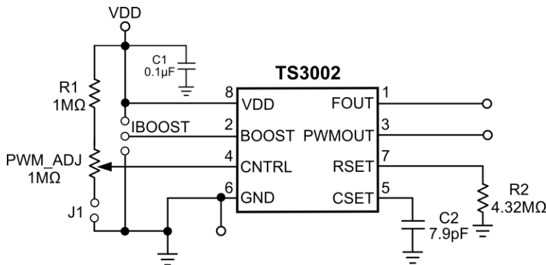
Figure 1. TS3002 Oscillator/Timer Circuit
