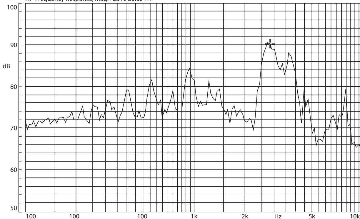
A: Frequency Response, Magn dB re 20.00 PA
