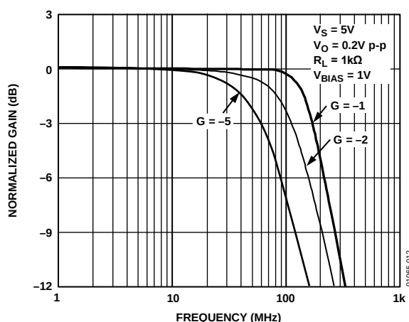
Figure 12. Small Signal Frequency Response
