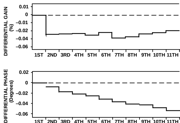
Figure 22. Differential Gain and Phase Error, G = 2 , NTSC Input Signal, R_L = 1k\Omega , V_S = 5V
