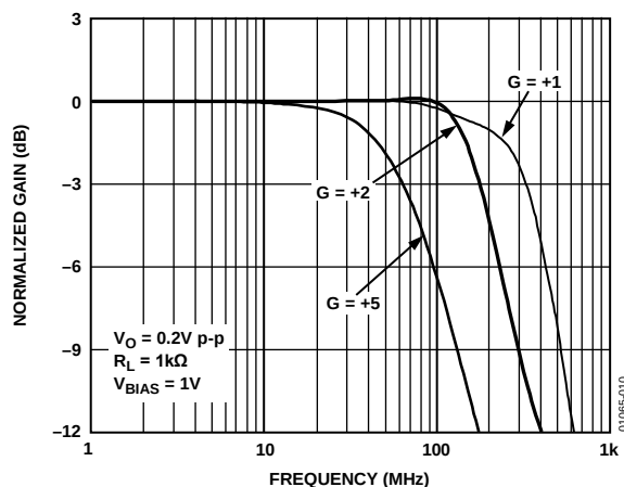
Figure 10. Small Signal Frequency Response
