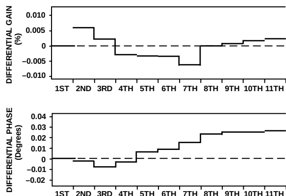
Figure 23. Differential Gain and Phase Error, G = 2 , NTSC Input Signal, R_L = 150\Omega , V_S = 5V
