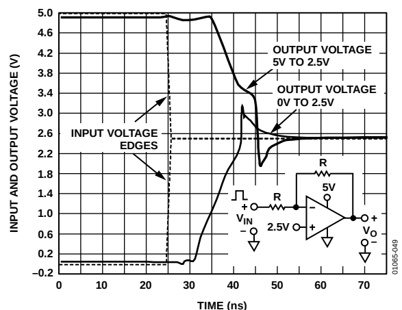
Figure 49. Overload Recovery, G = -1 , V_S = 5\text{ V}
