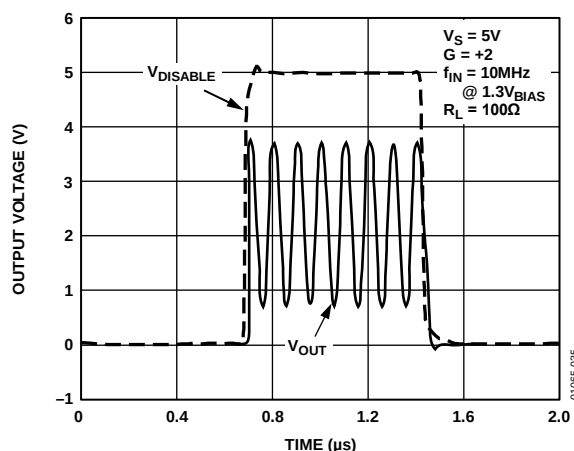
Figure 35. AD8063 \overline{DISABLE} Function, Voltage = 0 V to 5 V
