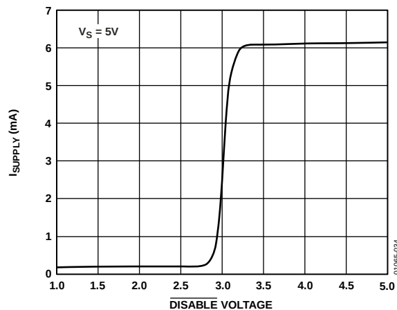
Figure 34. AD8063 \overline{DISABLE} Voltage vs. Supply Current
