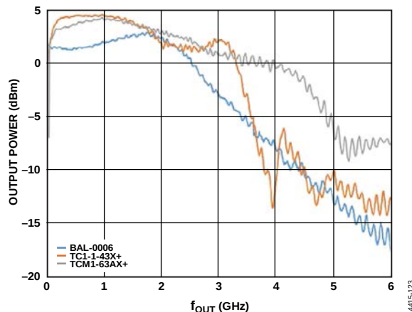
Figure 137. Measured DAC Output Response; f_{DAC} = 6 GS/PS
