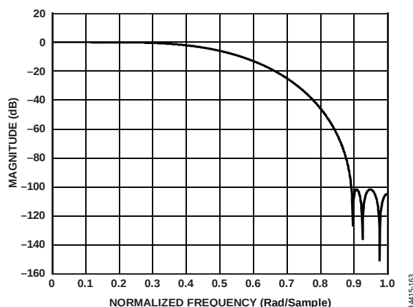
Figure 115. Third 2x Half-Band 22.5% Filter Response
