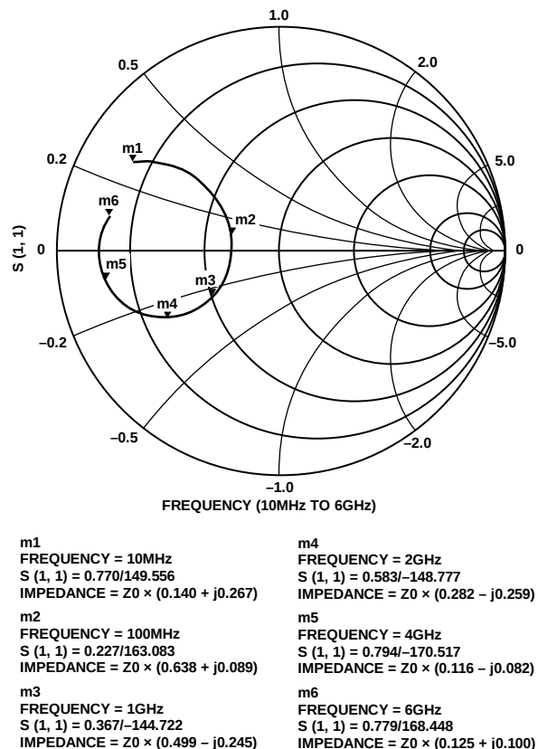
Figure 140. Simulated Smith Chart Showing the DAC Output Impedance, Z_0 = 100 \Omega
