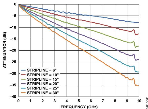
Figure 95. Insertion Loss of 50 \Omega Striplines on FR4
