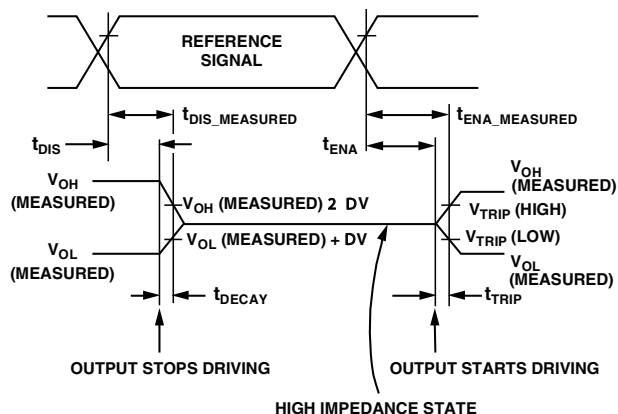
Figure 63. Output Enable/Disable
