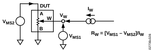
Figure 28. Wiper Resistance
