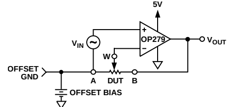
Figure 31. Noninverting Gain
