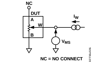
Figure 26. Resistor Position Nonlinearity Error (Rheostat Operation; R-INL, R-DNL)
