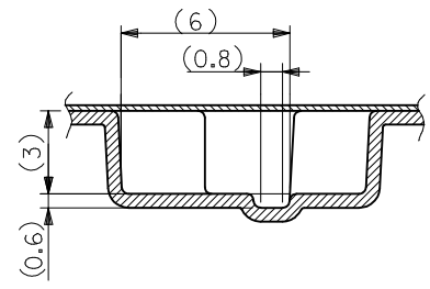
SECT:W-W
