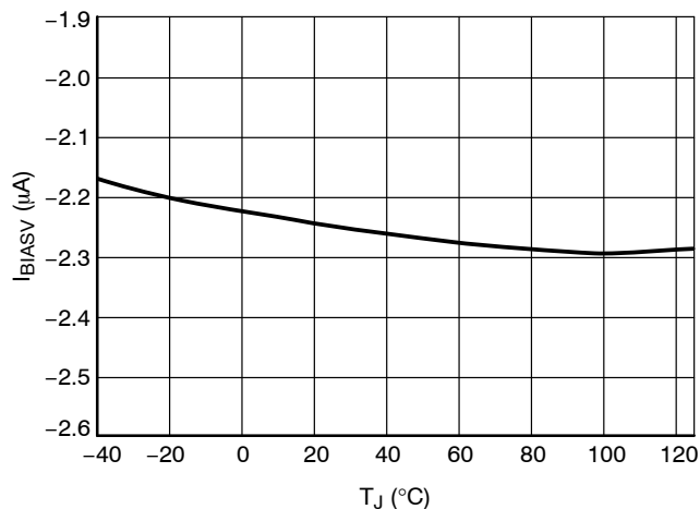
Figure 13. I BIASV at V CC = 15 V, V SNS > V SNSBIASHTH
