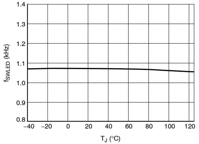
Figure 21. LED Switching Frequency at V_{CC} = 15\text{ V}
