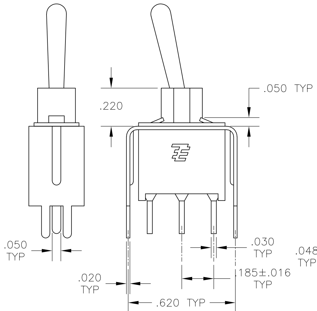
V30 V40 VERTICAL SUPPORT BRACKET
