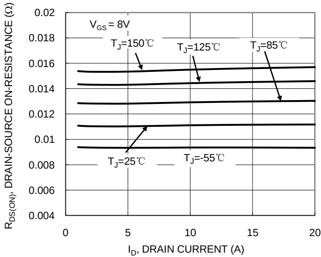
Figure 9. Typical On-Resistance vs. Drain Current and Junction Temperature
