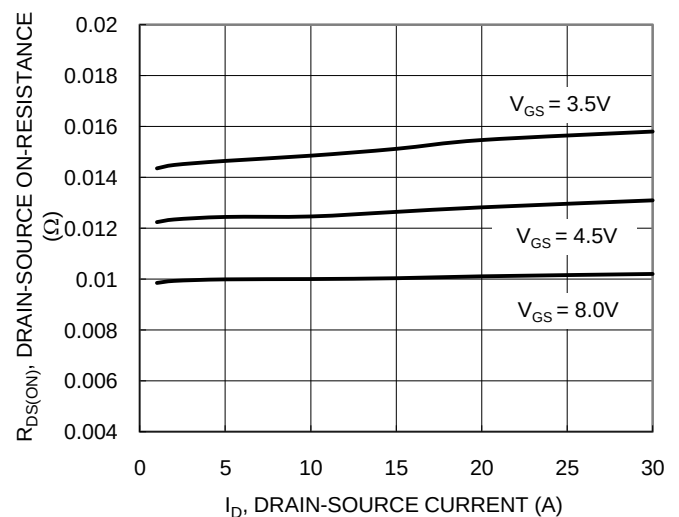
Figure 6. Typical On-Resistance vs. Drain Current and Gate Voltage
