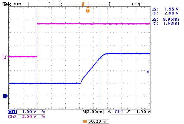
Figure 28: Turn on with Prebias 5V_{in}, 3.3V/OA out, V_{bias} = 1.0V_{dc}
