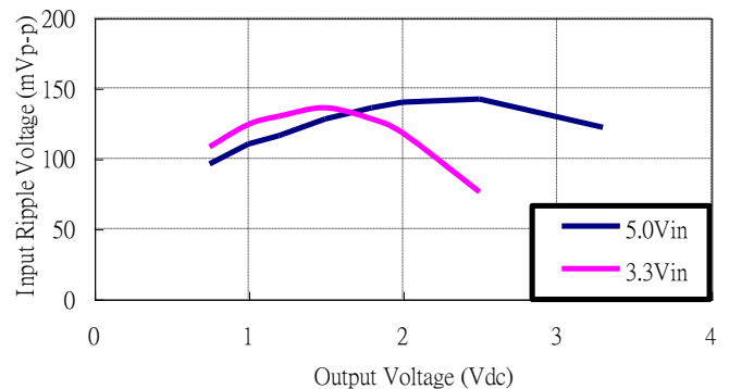
Figure 33: Input voltage ripple for various output models, I_O = 10 A ( C_{IN} = 4 \times 100 \mu F tantalum // 2 x 47 \mu F ceramic)
