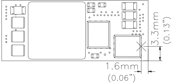
Figure 44: Temperature measurement location * The allowed maximum hot spot temperature is defined at 125°C
