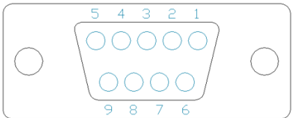
Figure 9: Serial DB9 Connector
