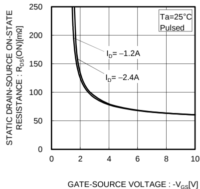
Fig.11 Static Drain-Source On-State Resistance vs. Gate-Source Voltage
