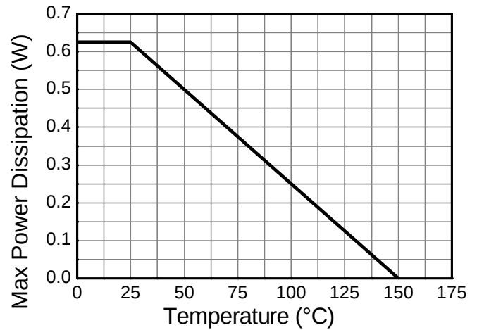
Derating Curve
