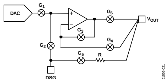
Figure 21. Block Diagram of AD7834/AD7835 Output Stage
