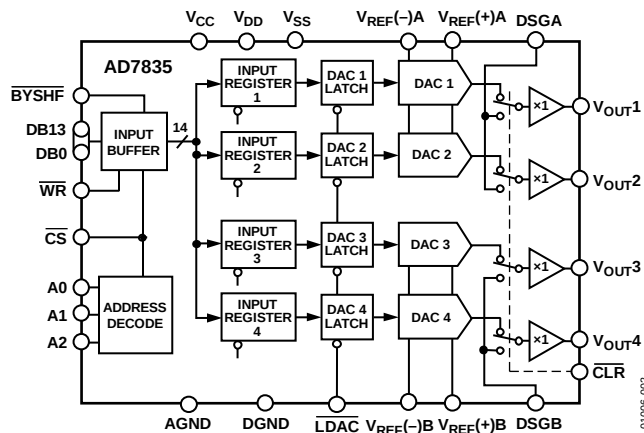
Figure 2. AD7835
