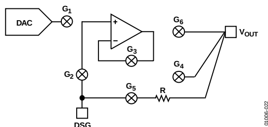
Figure 22. Output Stage with V_{DD} < 10\text{ V}
