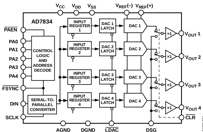
Figure 1. AD7834
