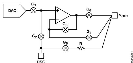
Figure 21. Block Diagram of AD7834/AD7835 Output Stage
