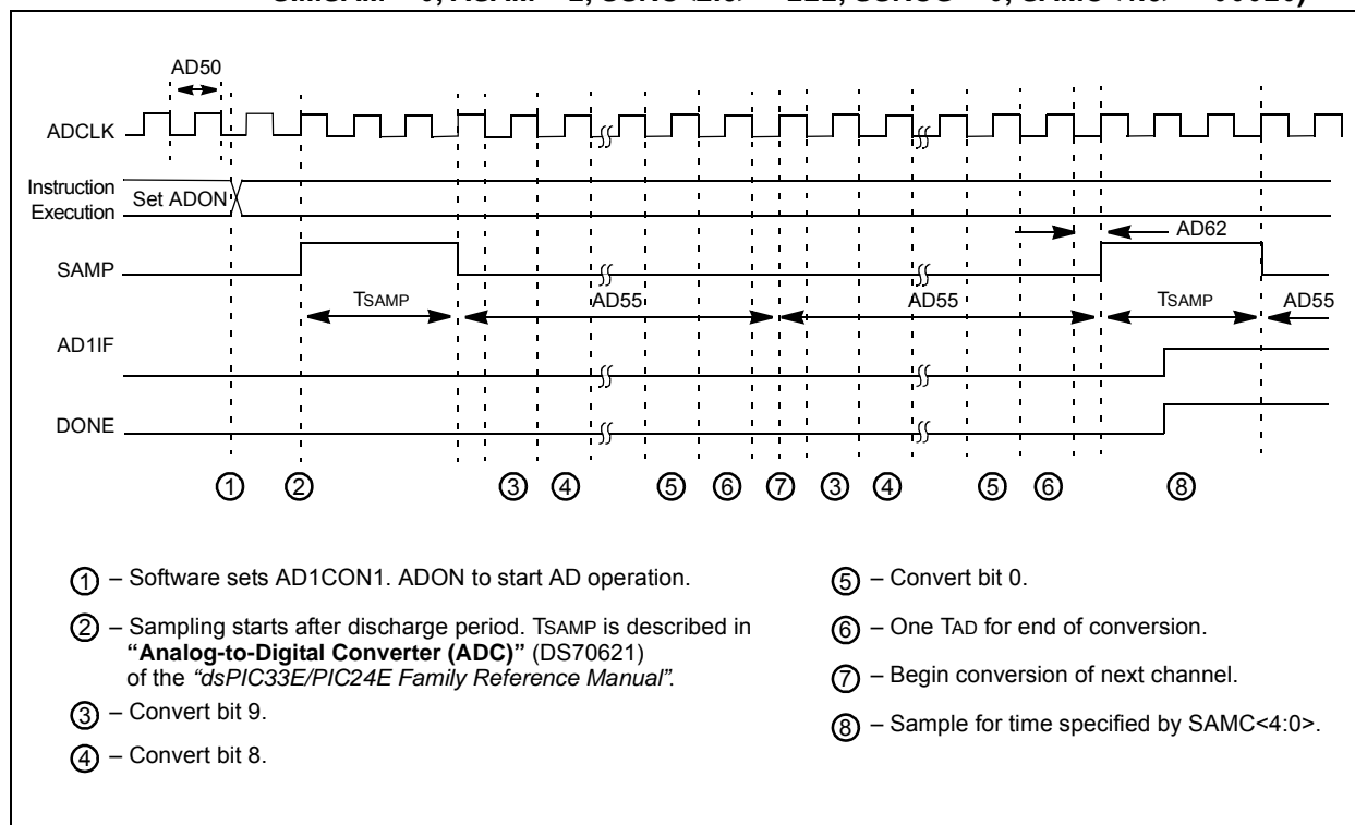
FIGURE 33-40: ADC CONVERSION (10-BIT MODE) TIMING CHARACTERISTICS (CHPS<1:0> = 01, SIMSAM = 0, ASAM = 1, SSRG = 0, SAMC<4:0> = 00010)
