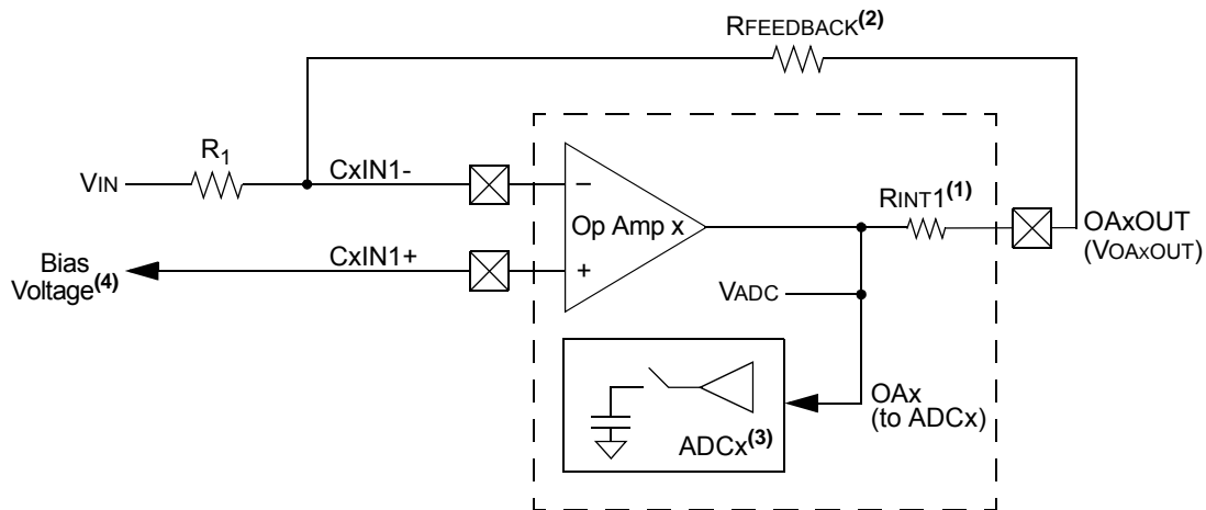
FIGURE 26-5: OP AMP CONFIGURATION A
