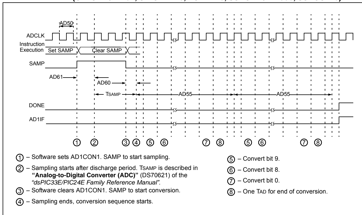
FIGURE 33-39: ADC CONVERSION (10-BIT MODE) TIMING CHARACTERISTICS (CHPS<1:0> = 01, SIMSAM = 0, ASAM = 0, SSRG = 0)
