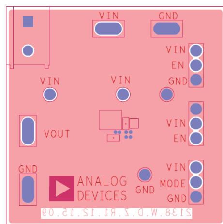
Figure 38. Bottom Layer
