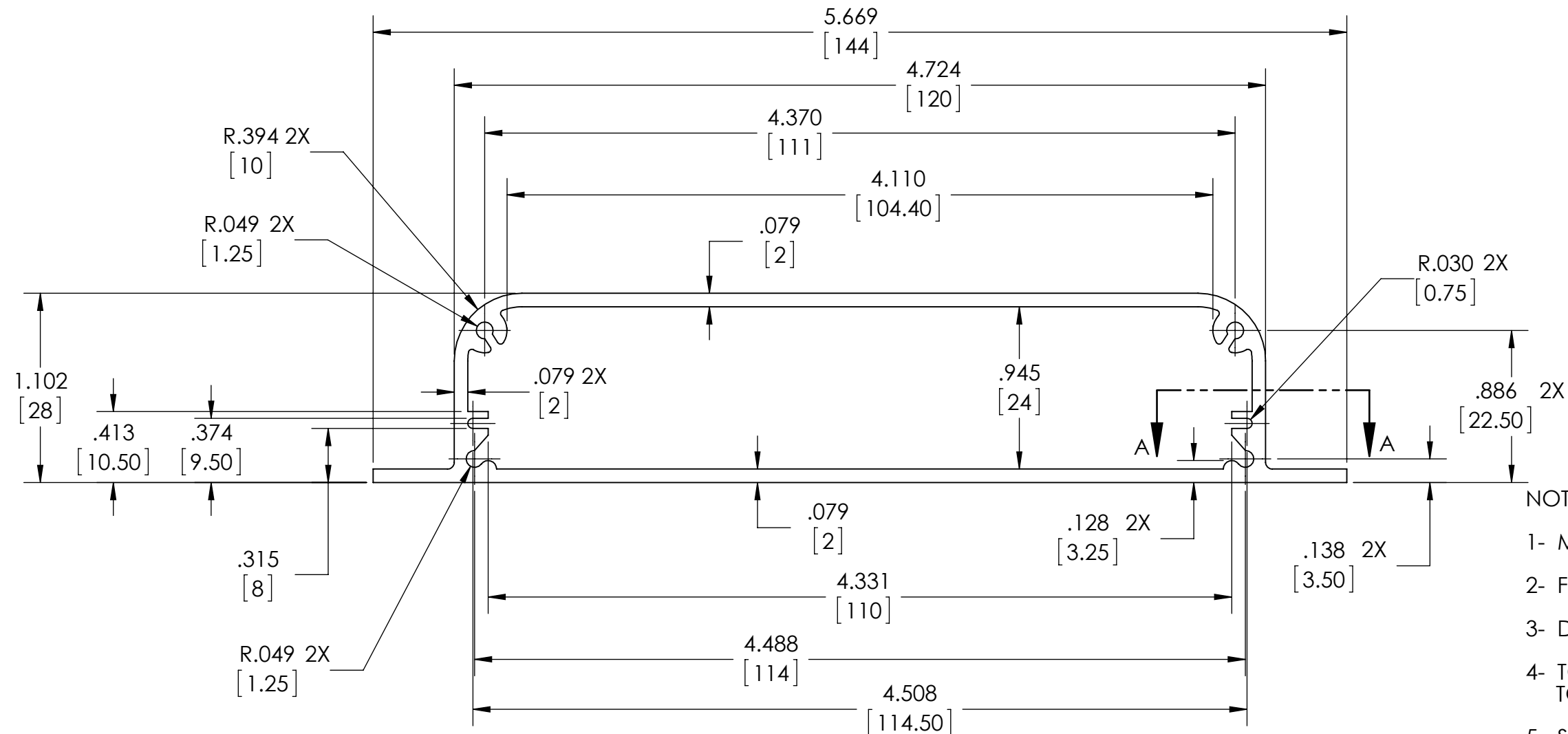
EXTRUSION PROFILE
