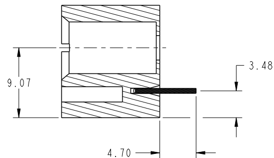
SECTION C-C SCALE 2:1
