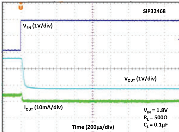
Fig. 33 - Turn-off Time
