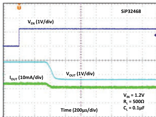
Fig. 32 - Turn-off Time
