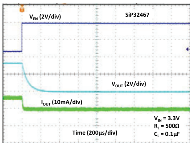
Fig. 29 - Turn-off Time
