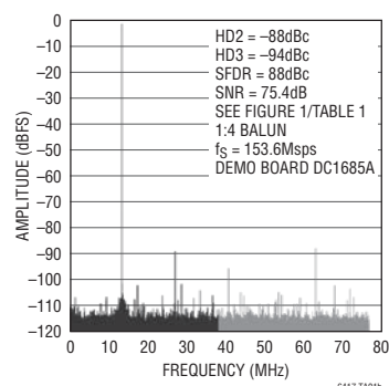
LTC6417 Driving LTC2209 16-Bit ADC 32K Point FFT, f_{IN} = 140\text{MHz} , -1\text{dBFS} , \text{PGA} = 0
