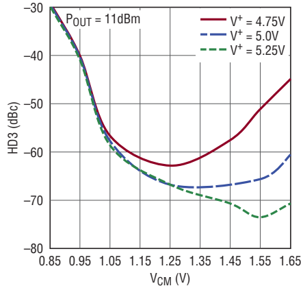
HD3 at 500MHz vs V_{CM} Over V^+
