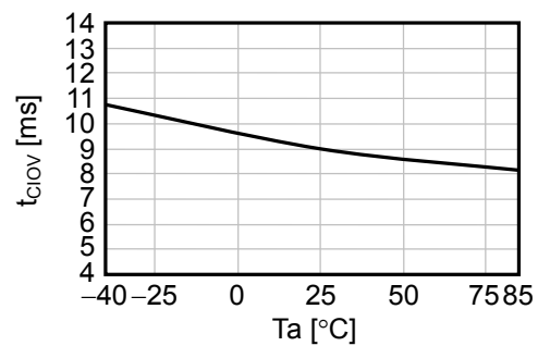
2.12 t_{CLOV} vs. T_a
