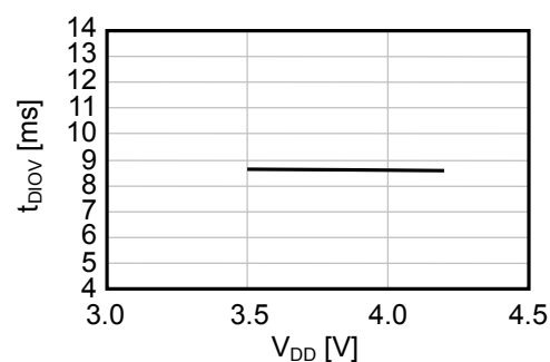
2.8 t_{DIOV} vs. V_{DD}
