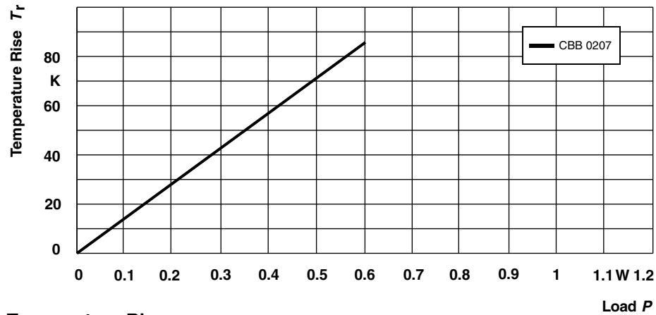
Temperature Rise
