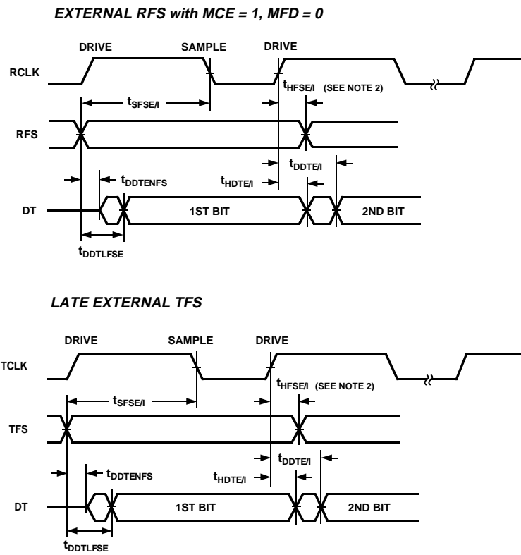
Figure 23. External Late Frame Sync
