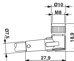
Dimensioned drawing
