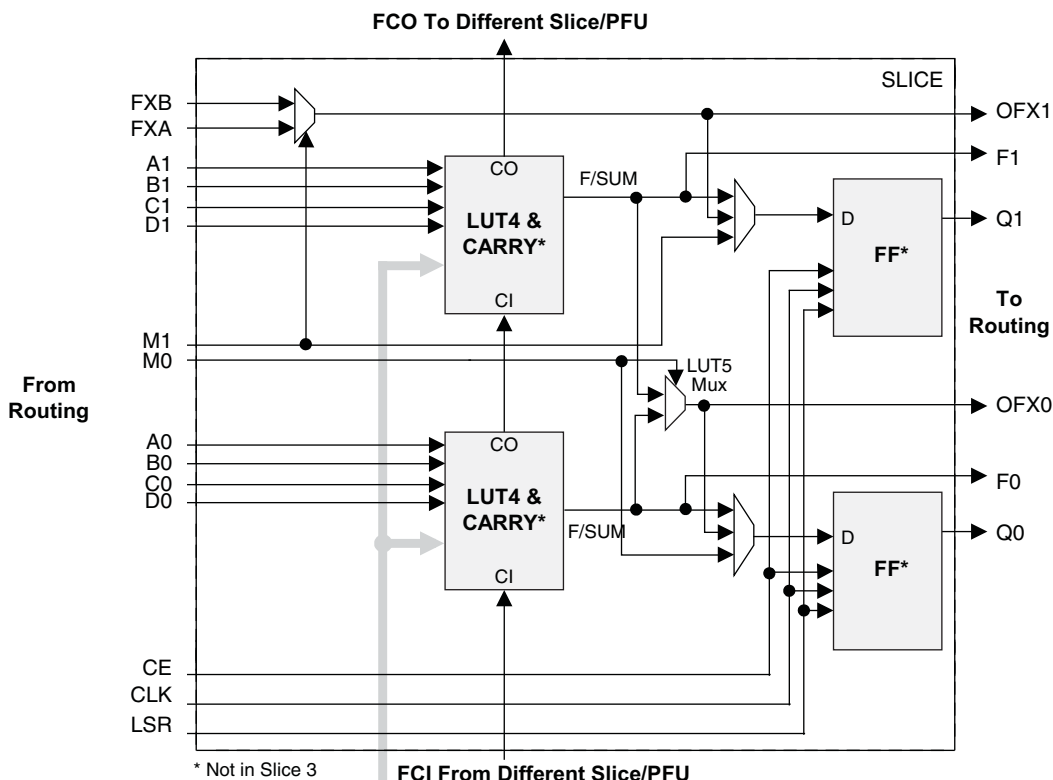
Figure 2-3. Slice Diagram
