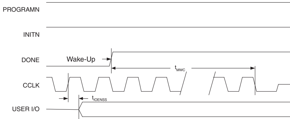
Figure 3-27. Wake-Up Timing
