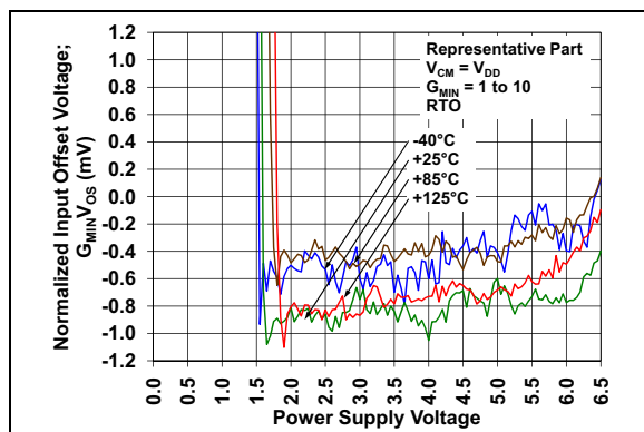
FIGURE 2-7: Normalized Input Offset Voltage vs. Power Supply Voltage, with V_{CM} = V_{DD} and G_{MIN} = 1 \text{ to } 10 .
