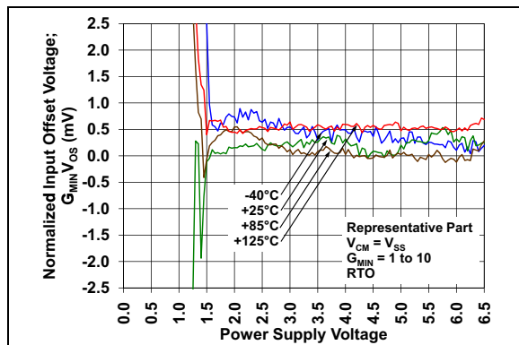
FIGURE 2-5: Normalized Input Offset Voltage vs. Power Supply Voltage, with V_{CM} = 0\text{V} and G_{MIN} = 1 \text{ to } 10 .
