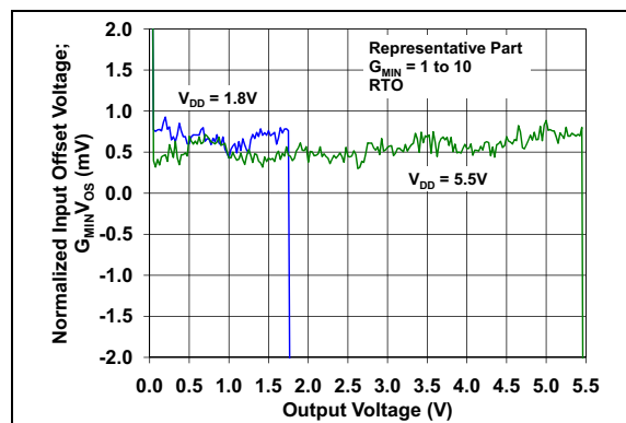
FIGURE 2-9: Normalized Input Offset Voltage vs. Output Voltage, with G_{MIN} = 1 \text{ to } 10 .
