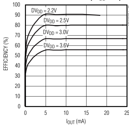
CHARGE-PUMP EFFICIENCY vs. OUTPUT CURRENT ( AV_{DD} = 4V )
