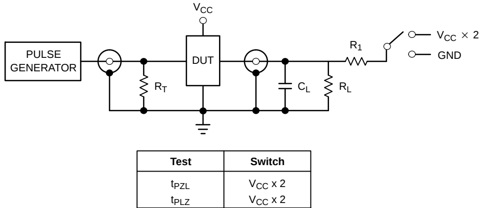
Figure 6. Test Circuit
