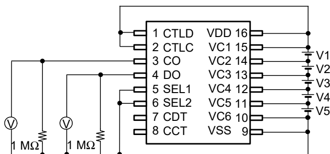
Figure 7 Test Circuit 4
