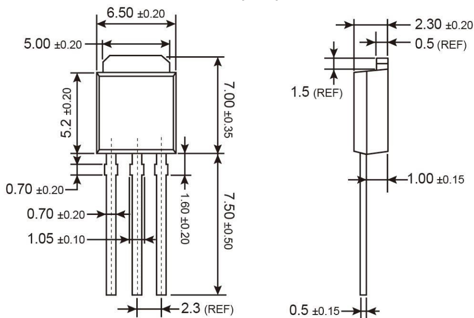
TO-251 (IPAK)
