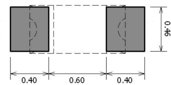
Figure 11: Recommended Solder Pad (Units: mm)
