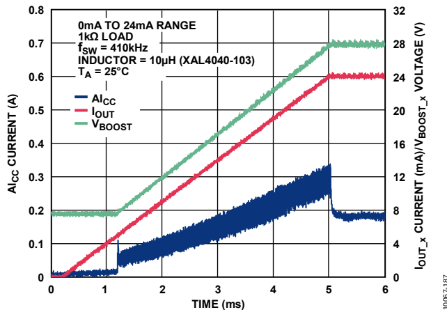
Figure 60. I_{CC} Current vs. Time for 24 mA Step Through 1 kΩ Load with Slew Rate Control
