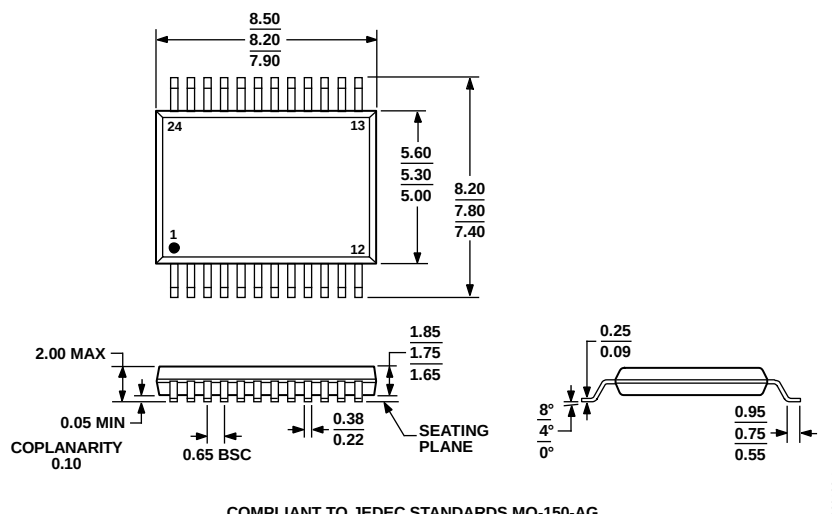
COMPLIANT TO JEDEC STANDARDS MO-150-AG Figure 34. 24-Lead Shrink Small Outline Package [SSOP] (RS-24) Dimensions shown in millimeters
