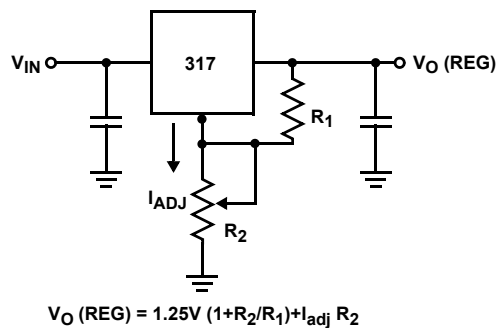
FIGURE 16. VOLTAGE REGULATOR
