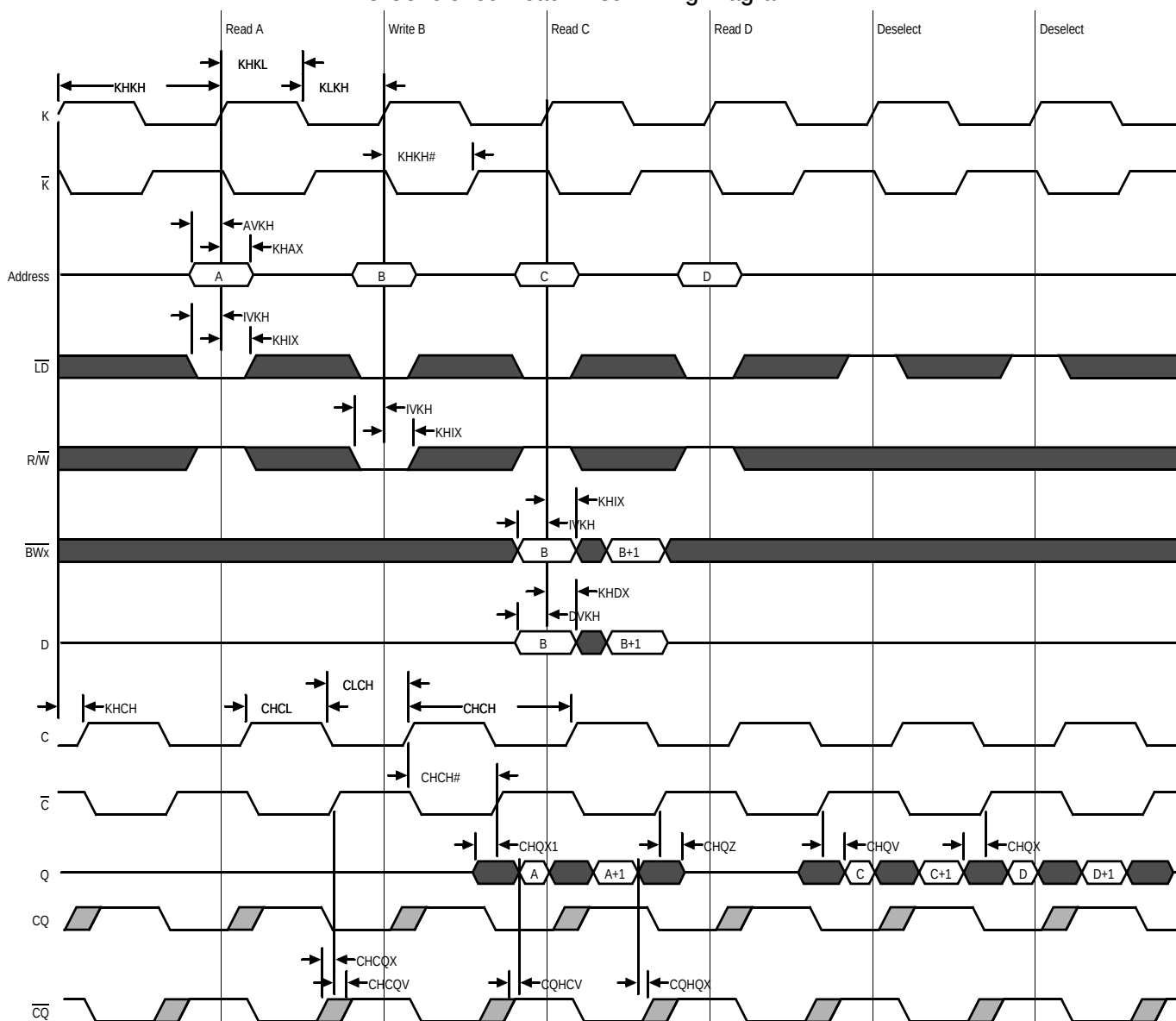
C Controlled Read-First Timing Diagram
