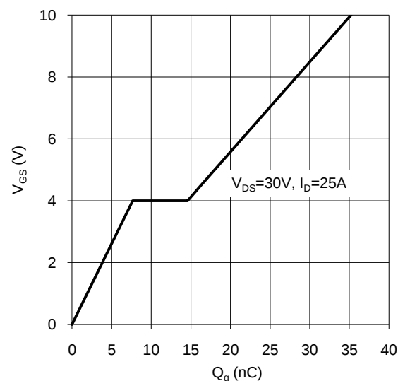
Figure 12. Gate Charge
