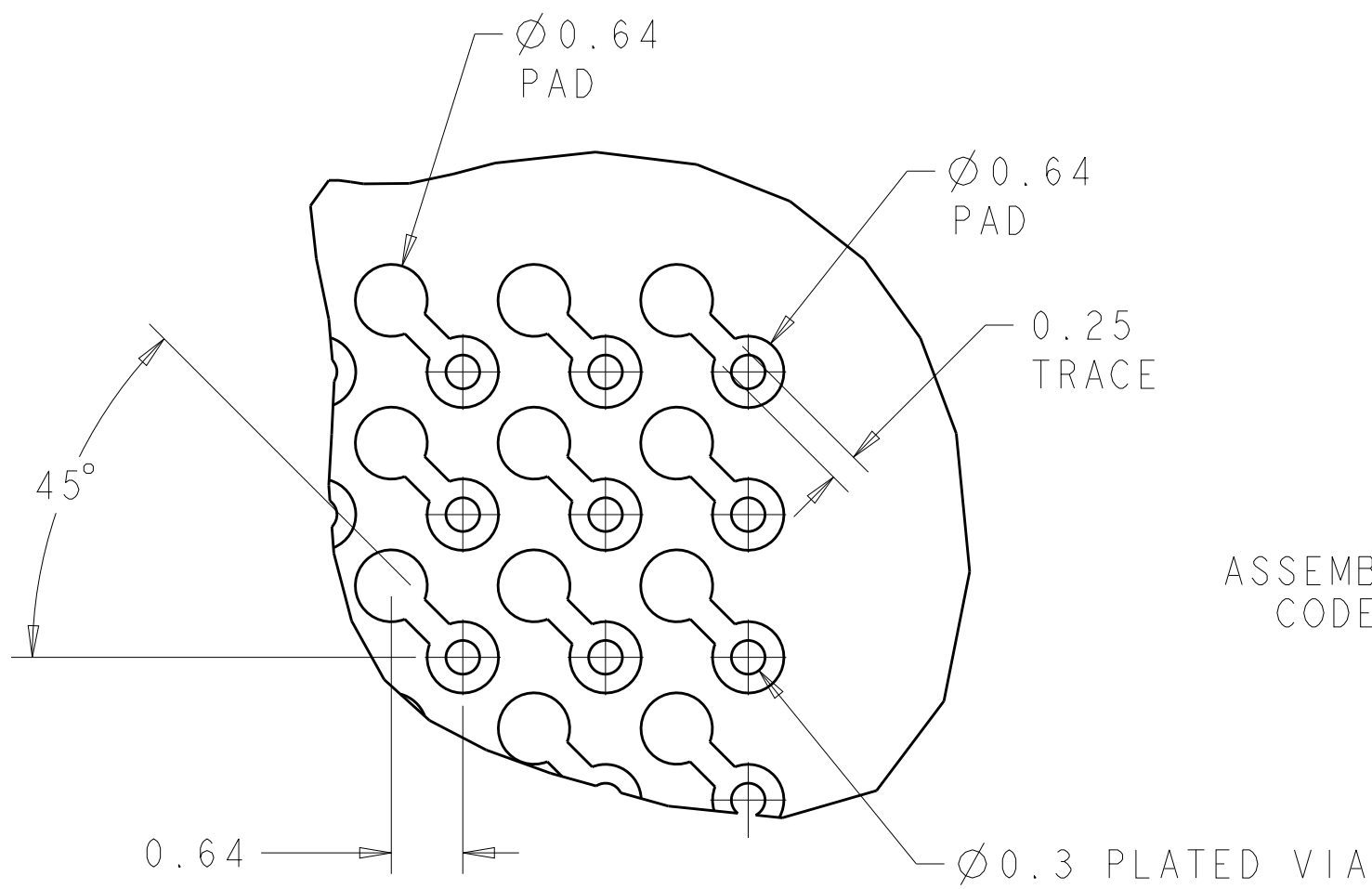
DETAIL X SCALE 16:1
