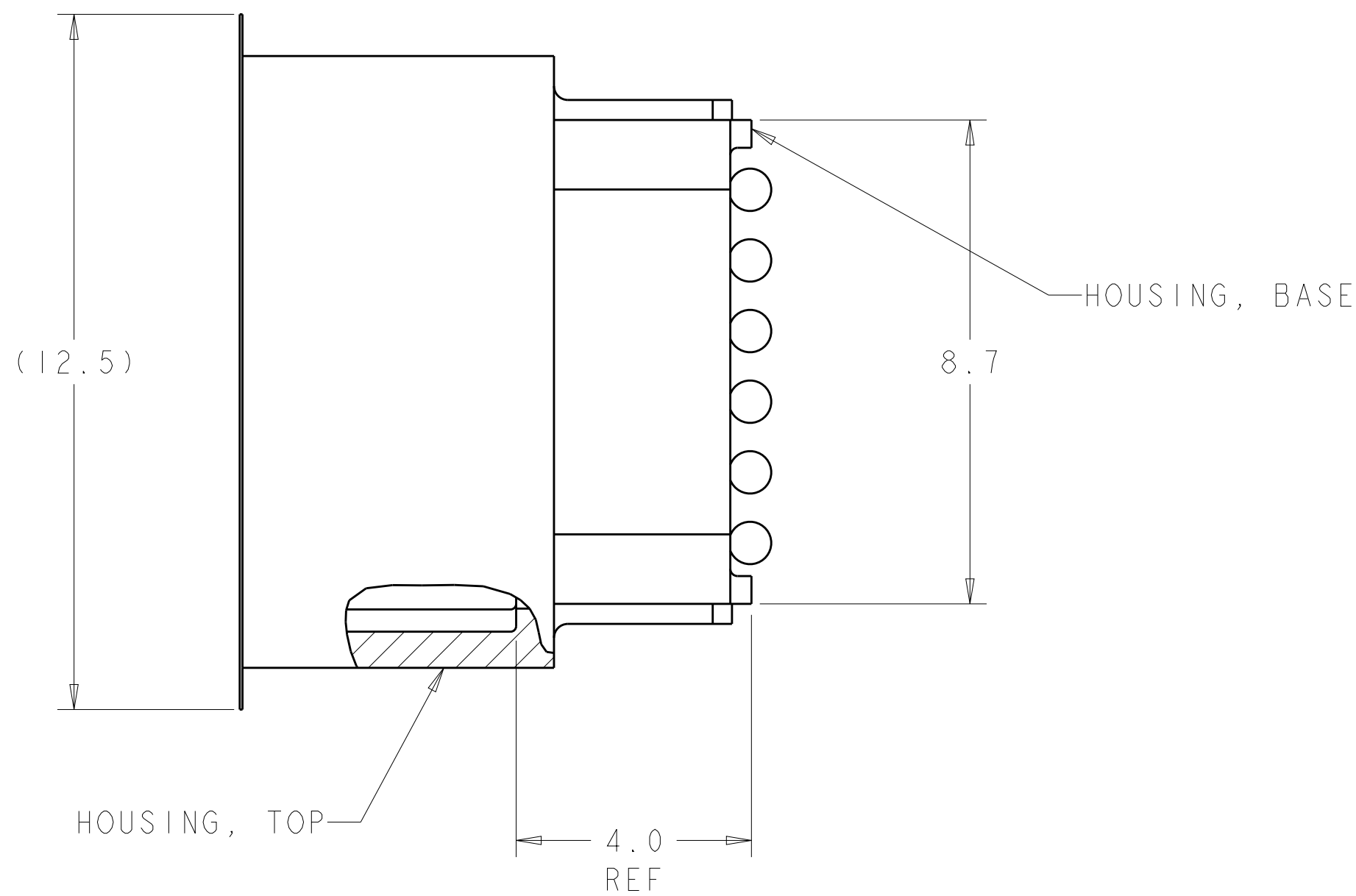
SECTION Z-Z
