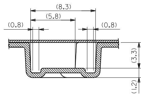
SECT. X-X
