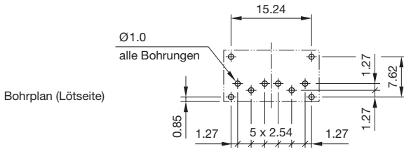
Component layout 1
