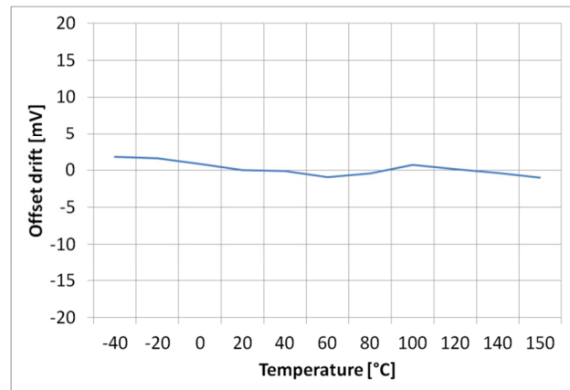
Figure 5: Thermal offset drift
